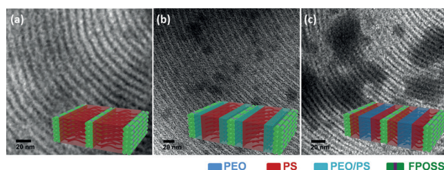
Figure 1. TEM BF images of curved lamellae of a) FPOSS-PS 36 , b) PS 38 -(FPOSS)-PEO 45 , and c) FPOSS-PS 48 - b -PEO 45 . The corresponding schematic models are included. All samples were stained with RuO 4 . Scale bars: 20 nm.
